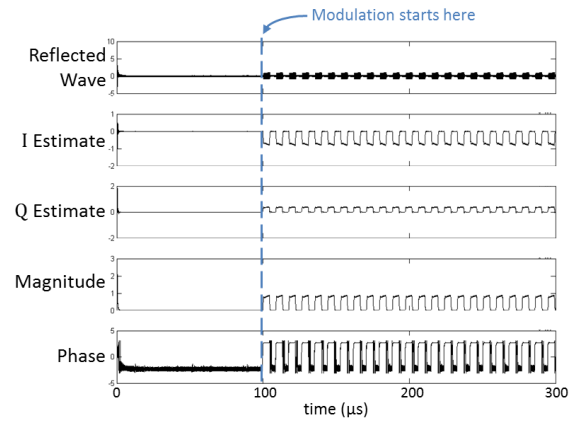
Fig. 4. The time domain response of the reflected signal (as seen at the directional coupler) is shown along with the extracted In-phase (I) and Quadrature (Q) components of that signal and the corresponding magnitude and phase values. Note that this work uses the vector distance between points on the IQ plane to decode transmitted data, similar to a conventional coherent radio receiver.
