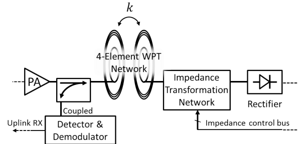
Fig. 1. A wireless power transfer system employing load modulation to transfer data from the power client to the power host. The effective load impedance is altered by a controllable impedance transformation network in order to produce detectable changes in the reflected signal. This work aims to optimize both load modulation capability and system efficiency.
