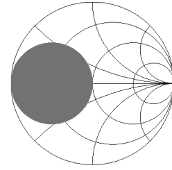
Fig. 3. The shaded region shows unattainable impedance values for the proposed pi-match topology and a capacitive rectifier load.
