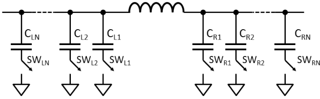
Fig. 2. The proposed switching pi-match topology allows for a wide range of impedance transformations. One switch configuration will produce the maximal efficiency case Z_{MATCH} , and another will correspond to the load modulation impedance Z_{LM} .
