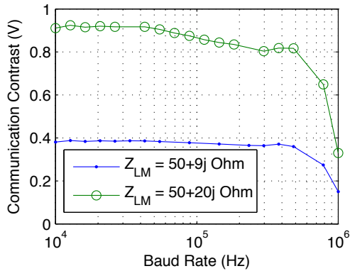
Fig. 9. Communication contrast (the distance between points on the IQ plane, in Volts) as a function of the load modulation baud rate (symbol rate), in Hz. With a typical binary shift keying modulation scheme, the data rate (bps) will be equivalent to the baud rate. Using higher order modulation schemes such as QAM allows multiplicative increases in data rate.
