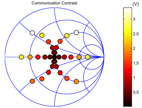
Fig. 7. Communication contrast (the distance between points on the IQ plane, in Volts) as a function of effective load modulation impedance Z_{LM} experienced at the power host's PA. The power client switches between Z_{MATCH} and Z_{LM} at a rate of 100 kHz.
