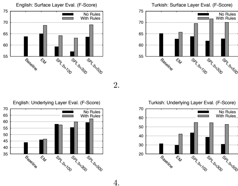
Figure 3: Development results for the preprocessed initial segmentation (Baseline), and segmentations produced by our approach, first after the EM Stage (EM) and again after the Split Stage (SPL) with different values of parameter b . Rules that generate underlying analyses have either been included (With Rules), or left out (No Rules).
